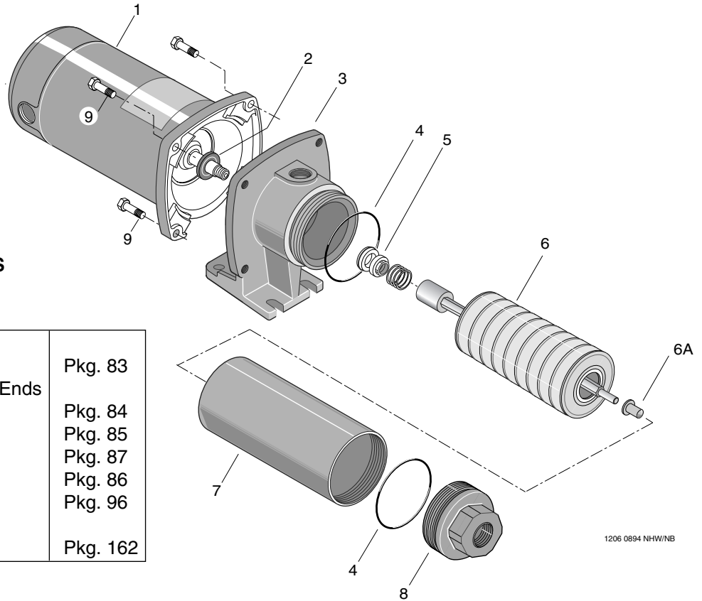
Figure 14 – Exploded view.
