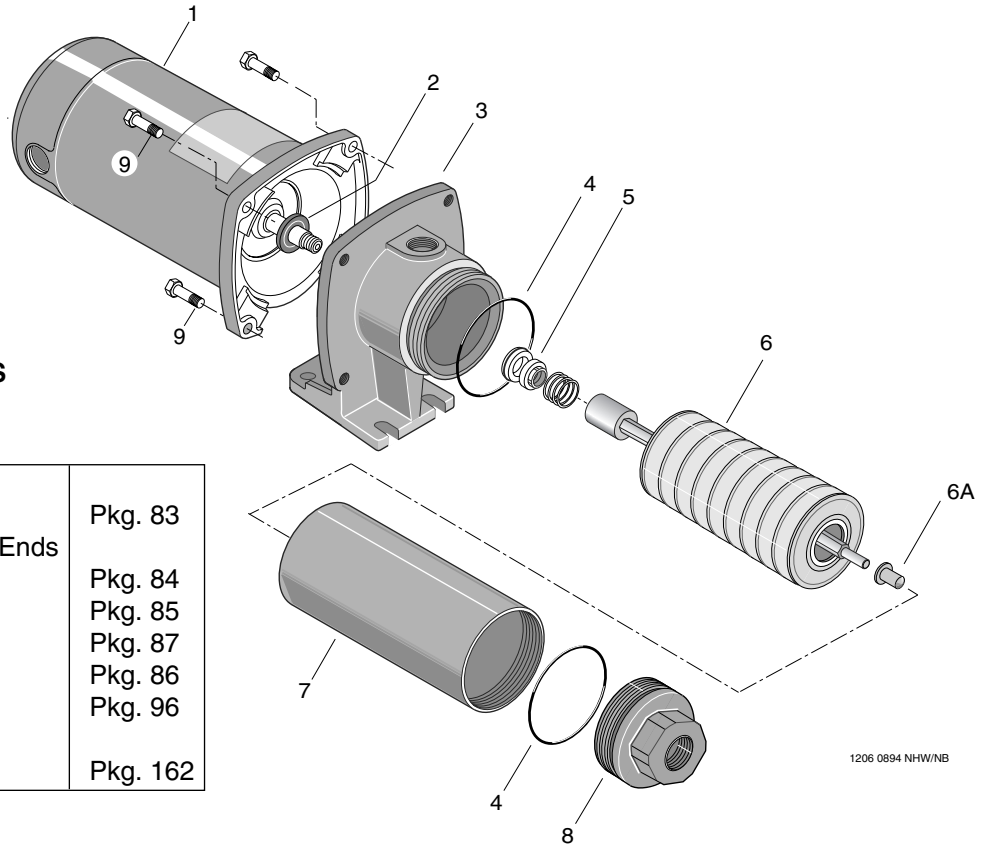
Figure 10 – Exploded view.
