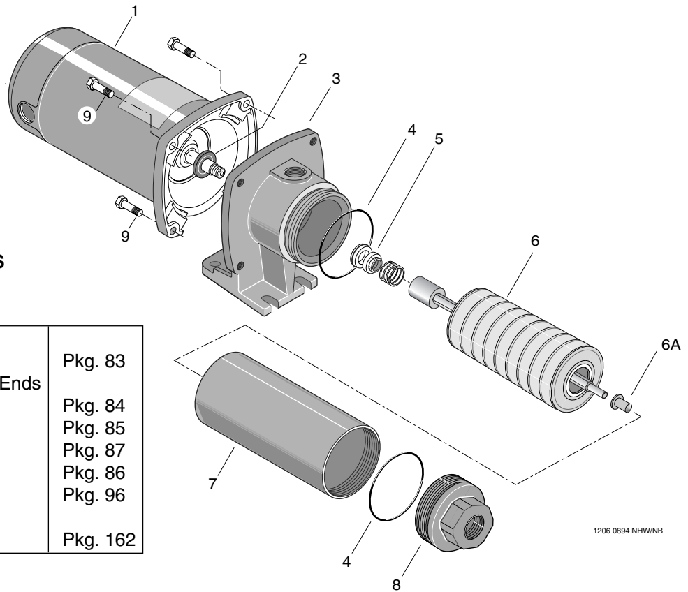
Figure 12 – Exploded view.
