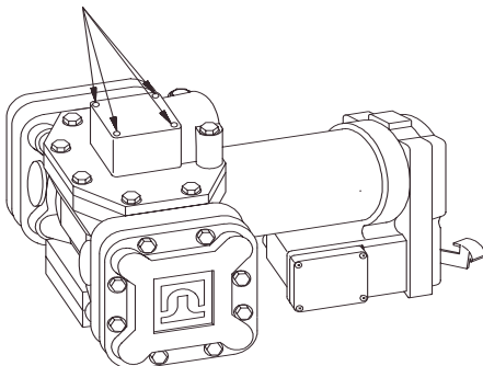
Mounting Holes
