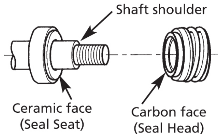
Figure 2 - Seal Installation
