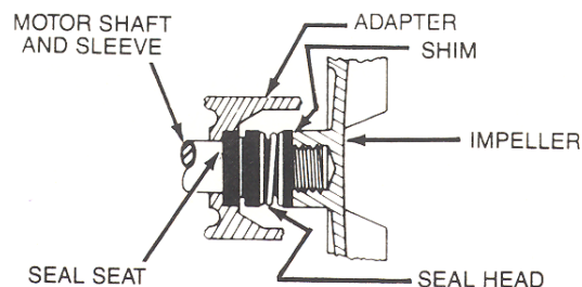
Figure 1 – Mechanical Seal
