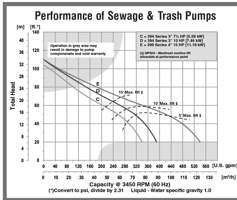
Figure 3 - Performance Curve
