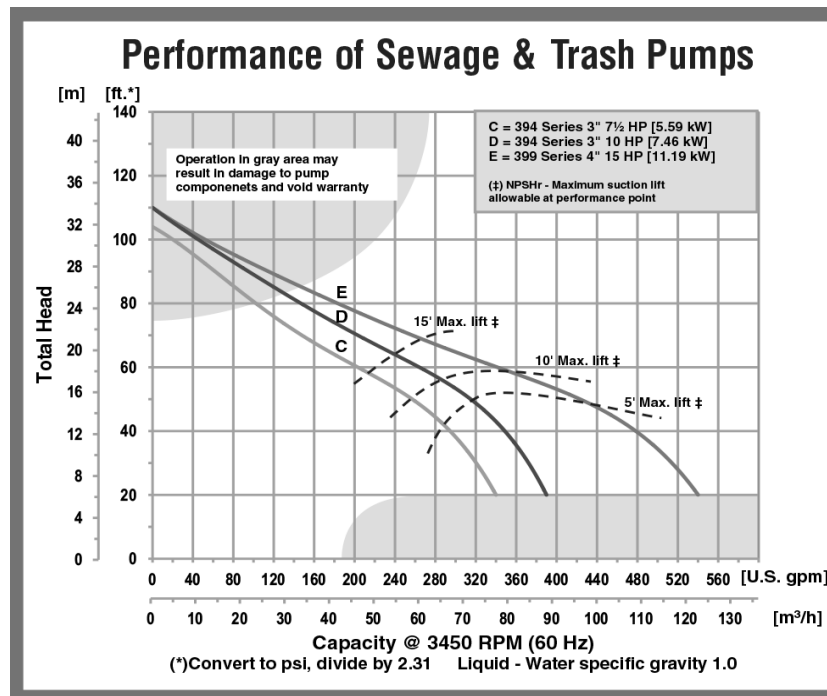
Figure 3 - Performance Curve
